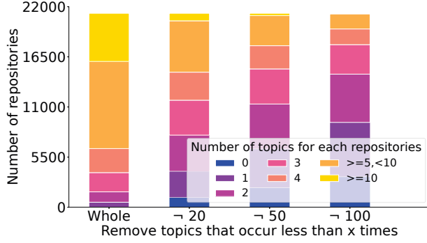
Fig. 2: Number of topics in repositories before and after removal of topics
