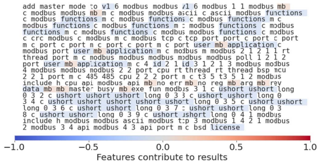
Fig. 5: Explanation for LR-TFIDF’s prediction on a repository with the correct topics: “modbus”, “master”, “freemodbus”
