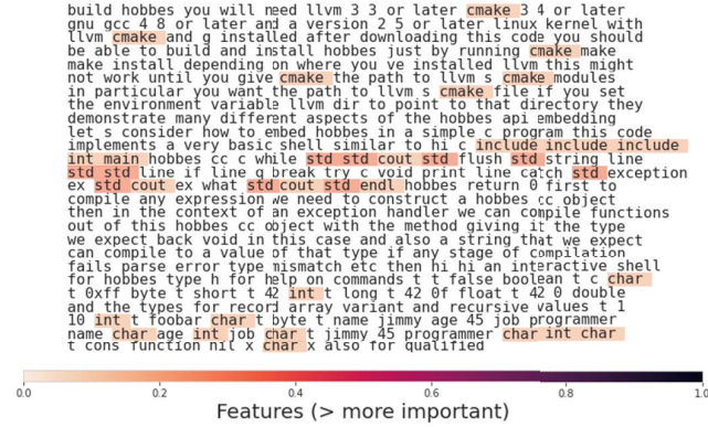
(a) Feature importance scores from LR-TFIDF. Its top-1 prediction is “cpp”
