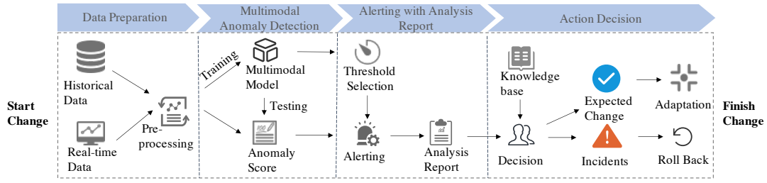
Figure 5: Overview of SCWarn
