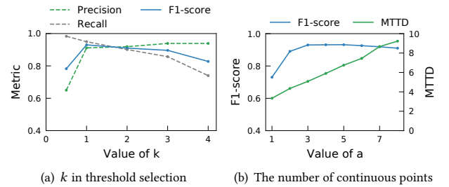
Figure 9: The effect of parameters
