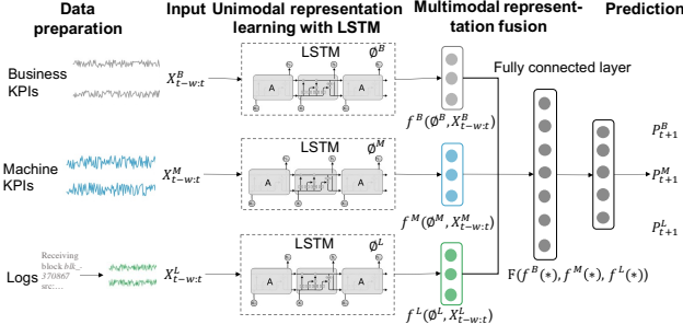
Figure 7: Multimodal anomaly detection model
