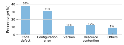
Figure 4: Percentage of different root causes
