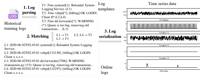
Figure 6: Illustration of log preprocessing
