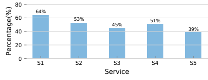
Figure 2: Percentage of incidents induced by changes
