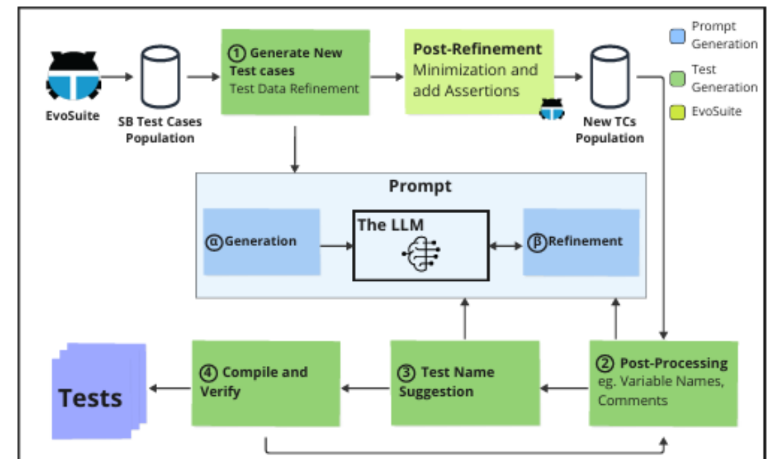
Fig. 2. Overview of the UTGen approach
