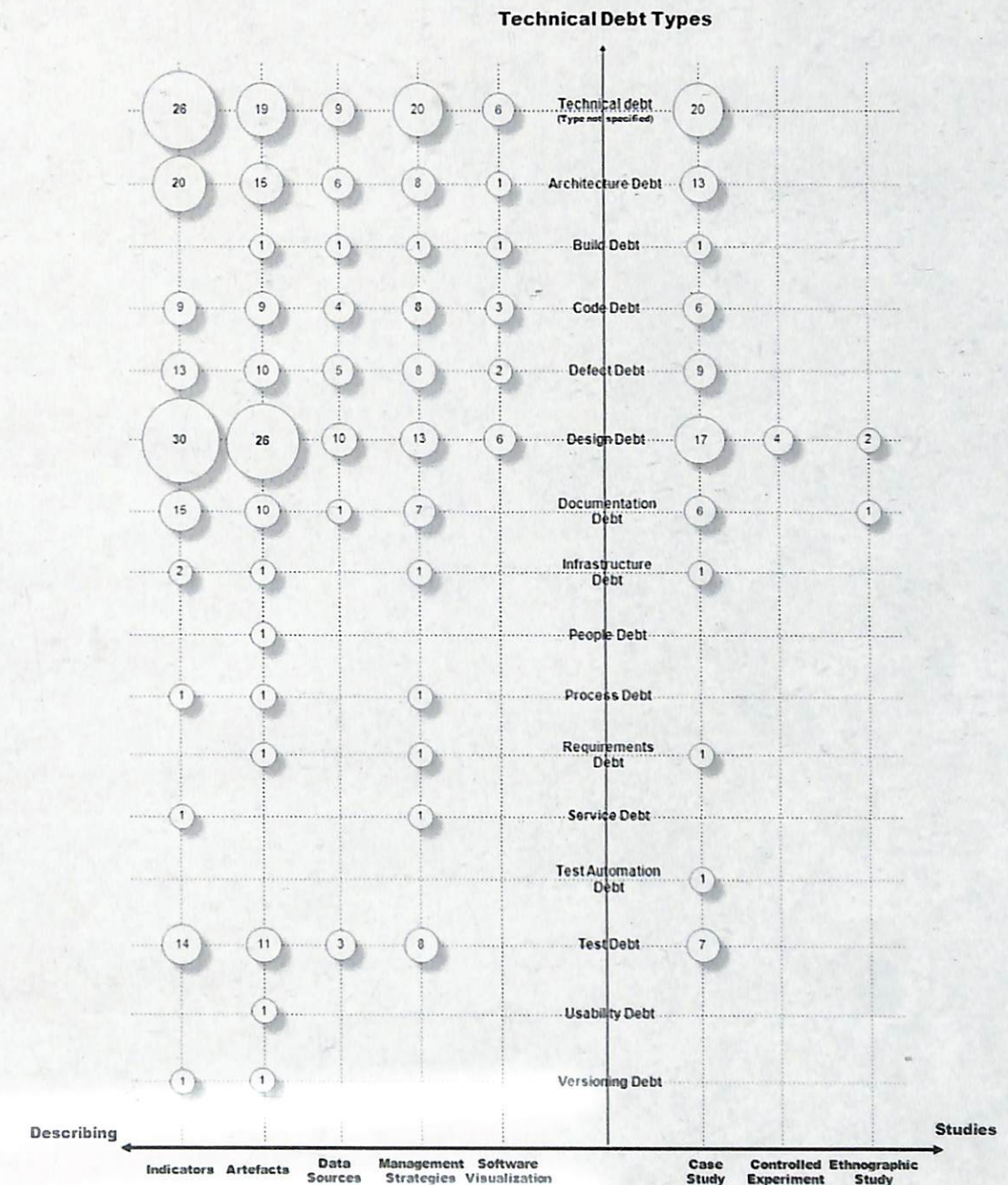
Fig. 13. A visualization of the systematic mapping in the form of a bubble chart.
