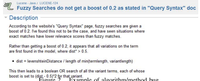
Figure 2. Example of algorithm/method bug
