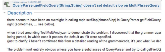
Figure 4. Example of assignment/initialization bug
